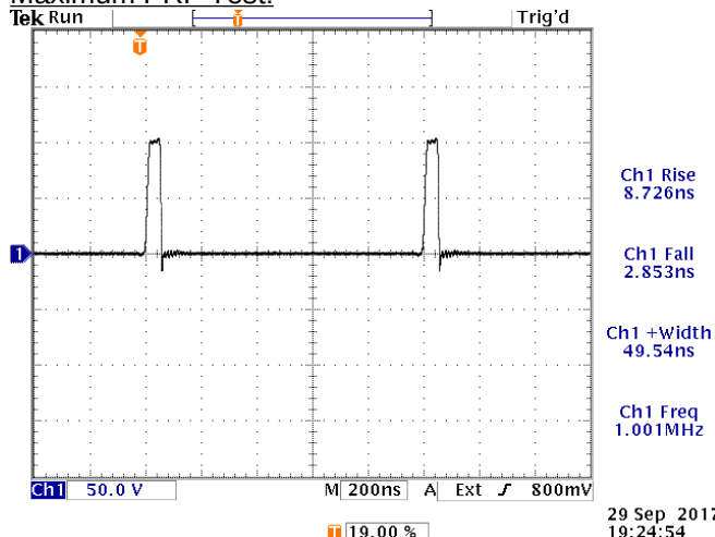
Output waveform (50V/div, 200 ns/div) for operation at 1 MHz, 50 ns, +100V.
