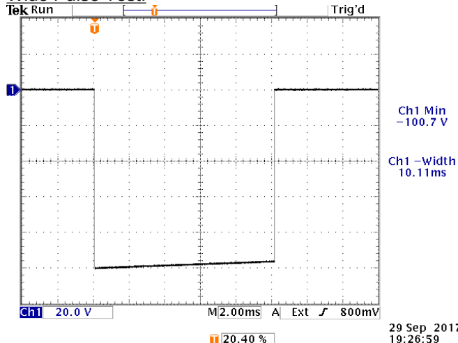
Output waveform (20V/div, 2 ms/div) for operation at 5 Hz, 10 ms, -100V.
