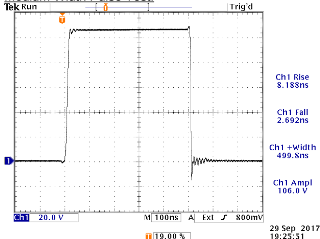
Output waveform (20V/div, 100 ns/div) for operation at 100 kHz, 500 ns, > +100V.
