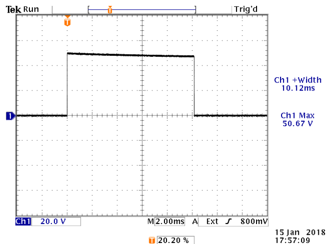
10 Hz, 10 ms, +50V, into 50 \Omega . 20V/div, 2 ms/div.
