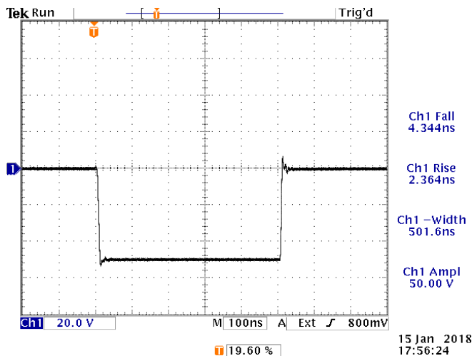
100 kHz, 500 ns, -50V, into 50 \Omega . 20V/div, 100 ns/div.
