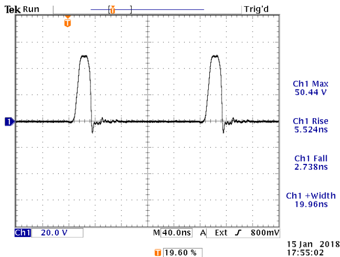
5 MHz, 20 ns, +55V, into 50 \Omega . 20V/div, 40 ns/div.
