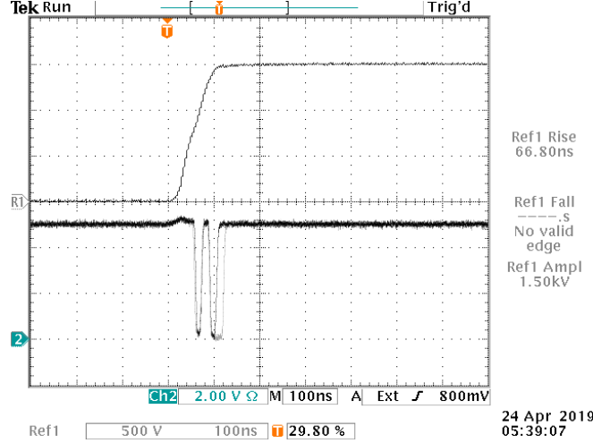
HCPL-7721, +5V input, +1.5 kV, +5V VCC2
