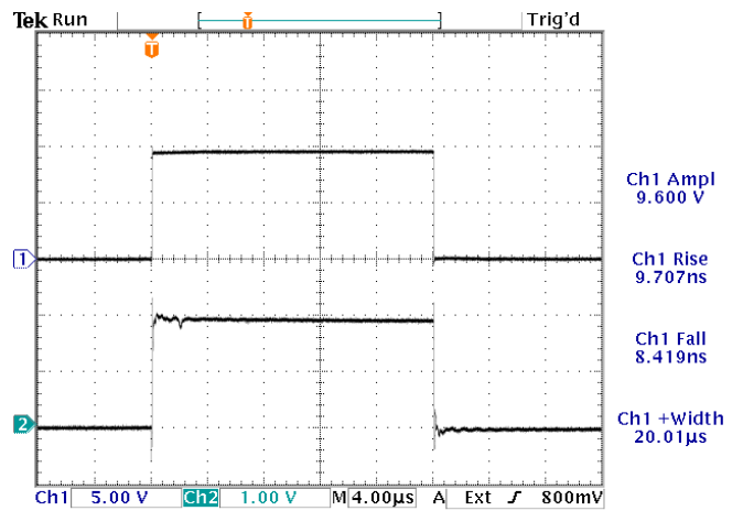
18 Apr 2023 10:36:34 Top: +10A into the supplied AV-CTL1-ENC test load (0.954 Ohms). 20 us pulse width. Bottom: MON MAX P monitor output into 50Ω.
