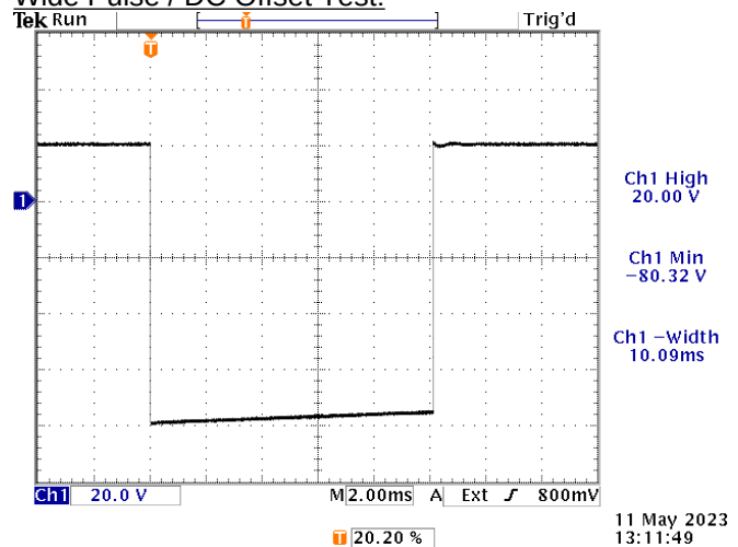
5 Hz, 10 ms, -100V, +20V offset. 20V/div, 2 ms/div.
