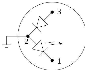
BOTTOM VIEW OF G1 PACKAGE
