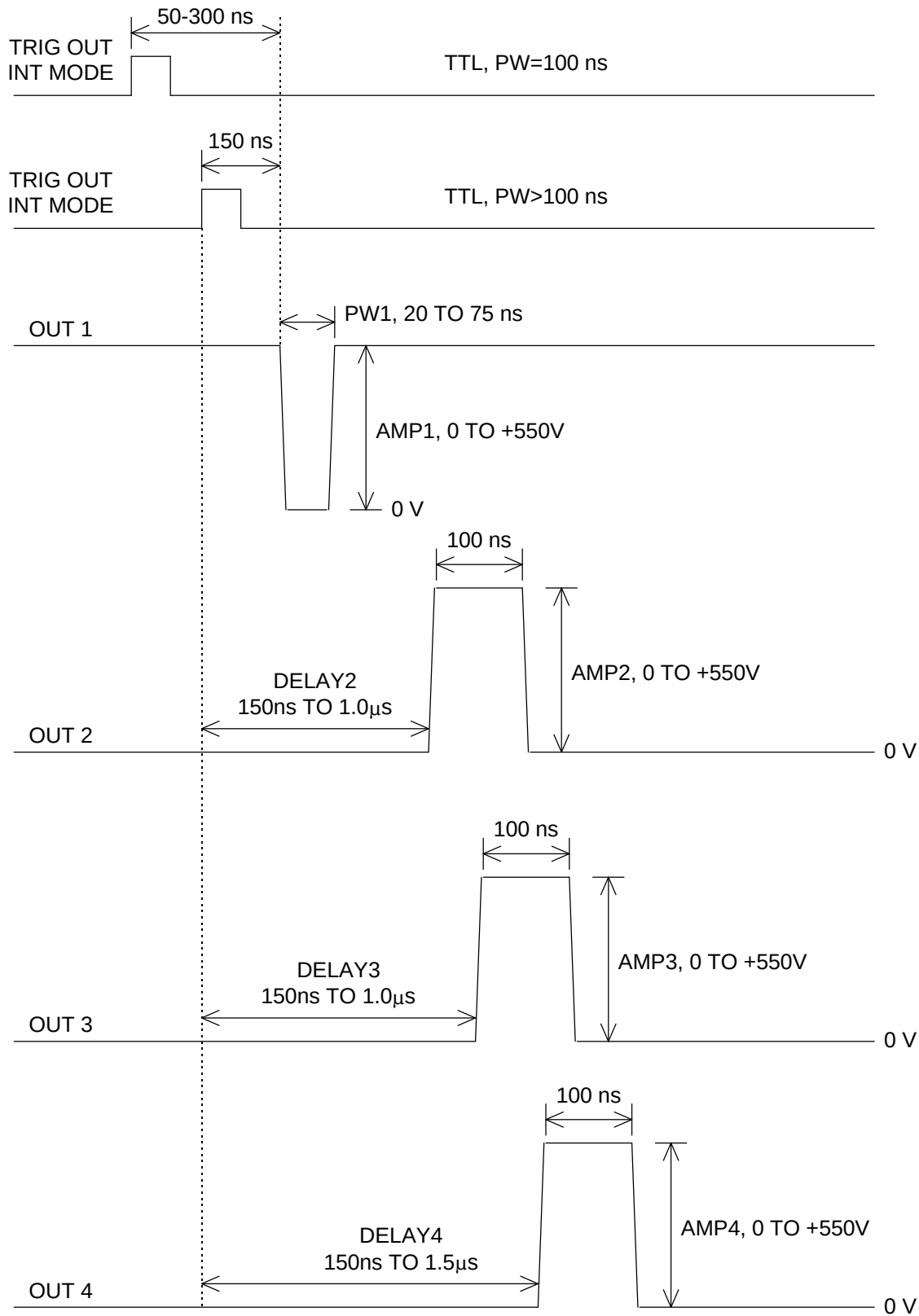
FIG 2 - TRIGGER WAVEFORMS AND AVX-M1 OUTPUT WAVEFORMS
