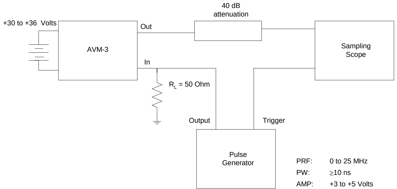
FIG. 1: PULSE GENERATOR TEST ARRANGEMENT
