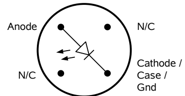
MATCHING USER-SUPPLIED DIODE PACKAGE (TOP VIEW). TO-46 PACKAGE.
