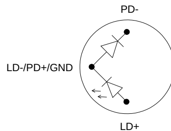
MATCHING USER-SUPPLIED DIODE PACKAGE (BOTTOM VIEW)
