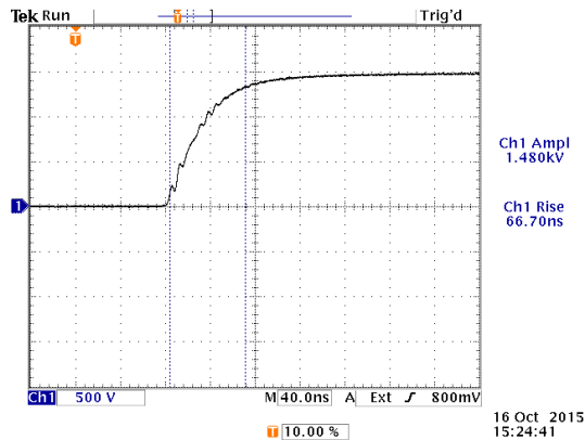
C = 300 pF, t_{R10-90} = 66.70 ns
