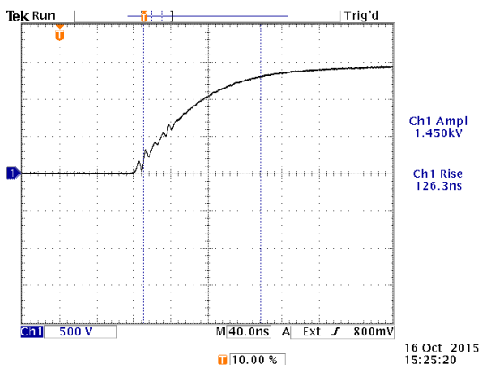
C = 600 pF, t_{R10-90} = 126.3 ns
