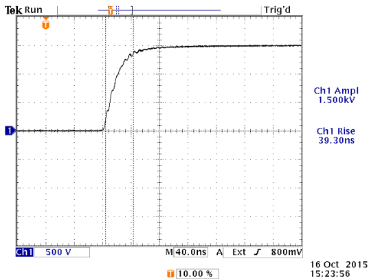
C = 150 pF, t_{R10-90} = 39.30 ns
