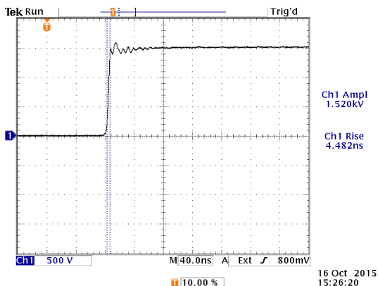
C = 0 pF, t_{R10-90} = 4.482 ns
