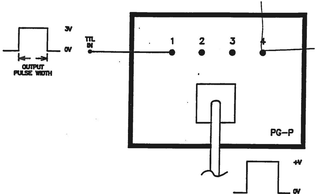
FIG. 10 POSITIVE PULSE GENERATOR MODULE
