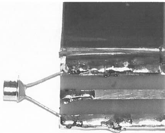
Wrong Way To Connect a Diode. The leads are too long!
