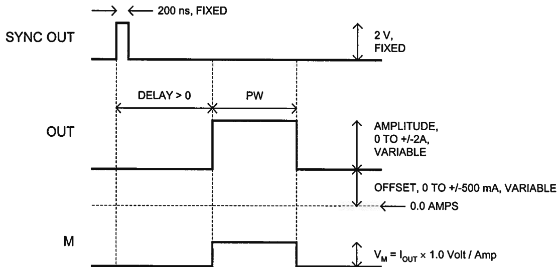
Basic Output Pulses for Delay > 0
