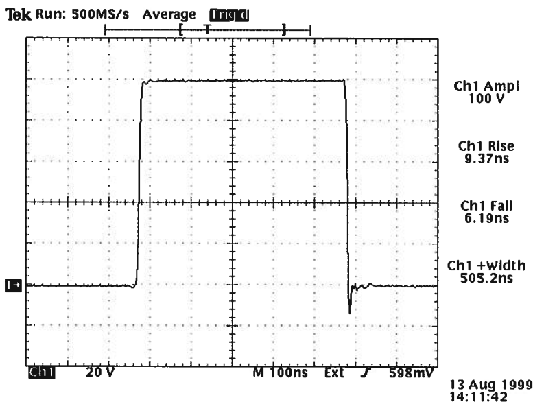
Figure 1 (20V/div, 100 ns/div)
