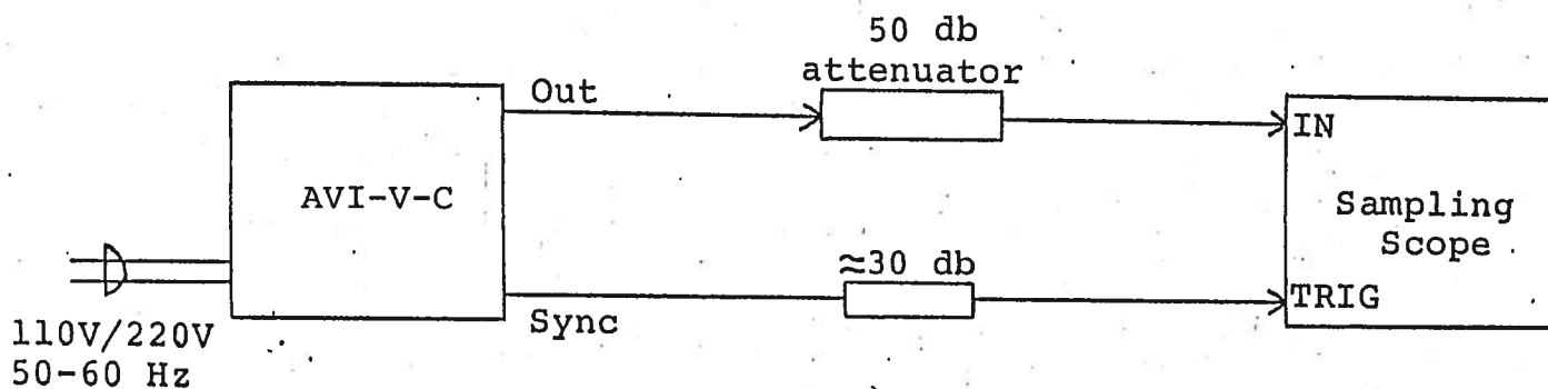
Fig. 1 PULSE GENERATOR TEST ARRANGEMENT
