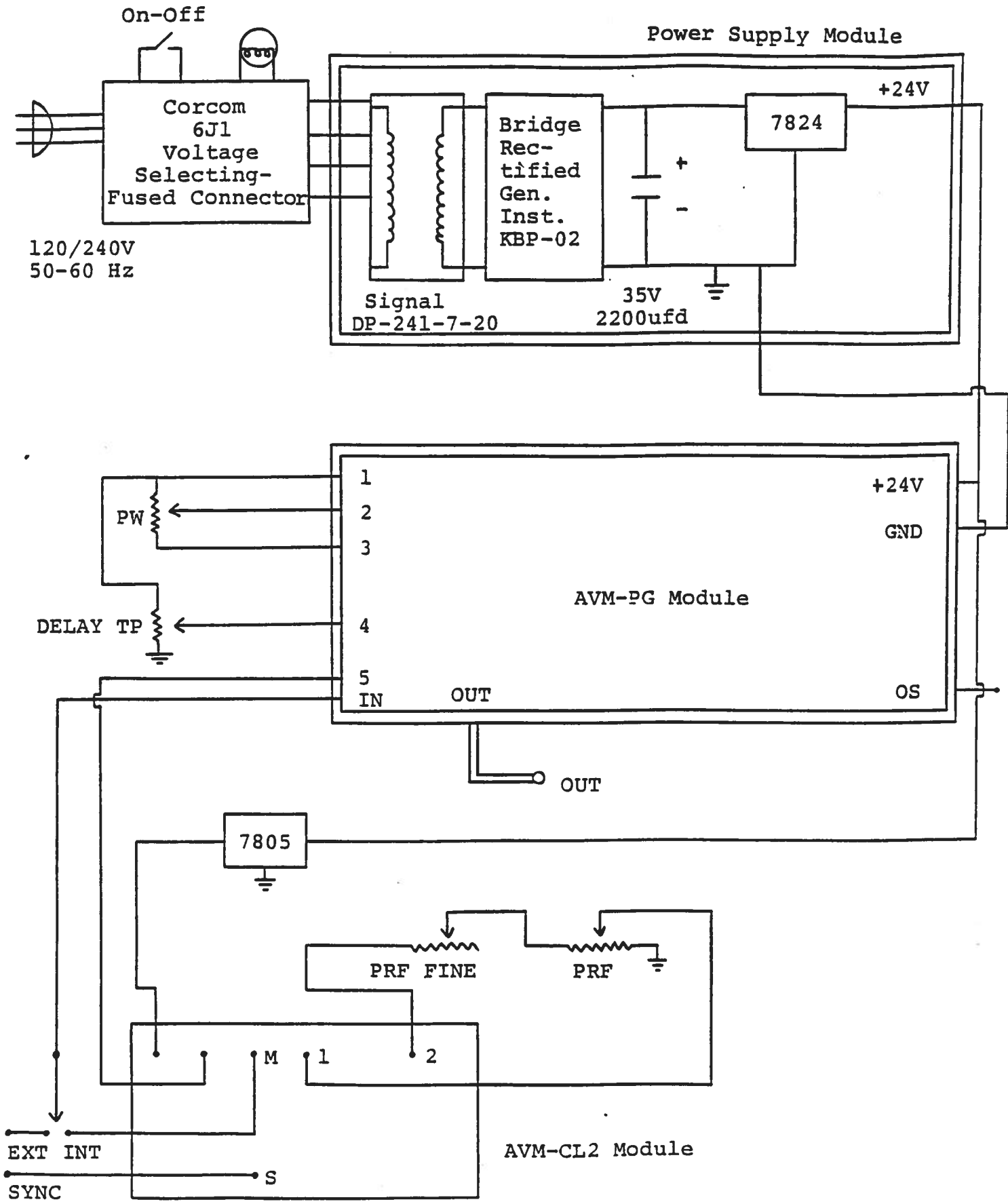
FIG. 4: SYSTEM BLOCK DIAGRAM
