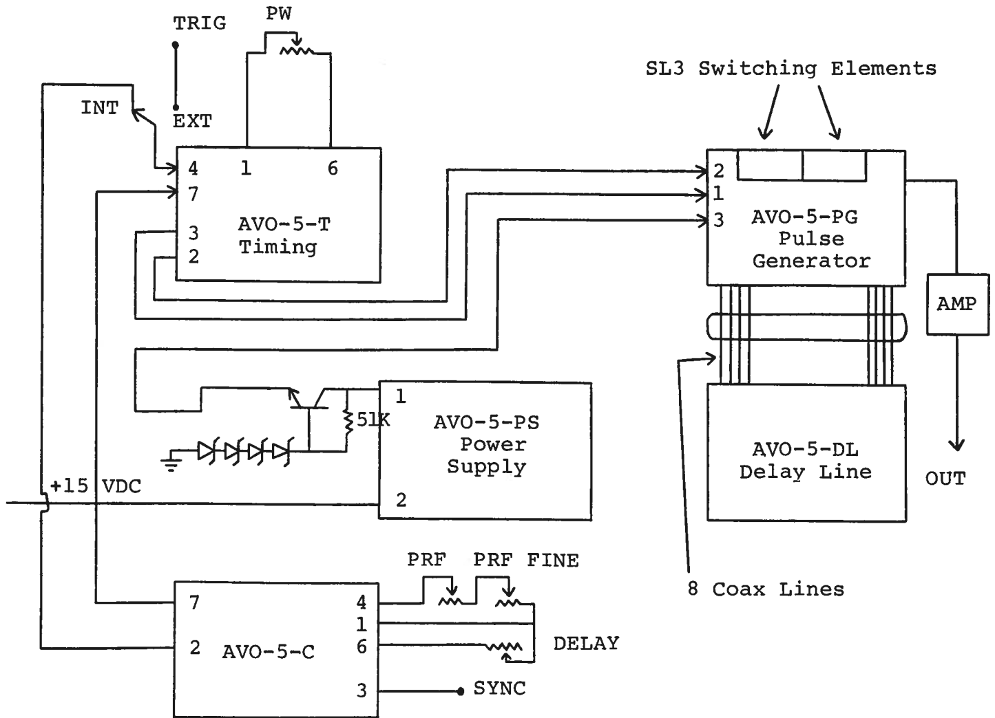
Fig. 4 System Block Diagram With Wiring and Pin Connections
