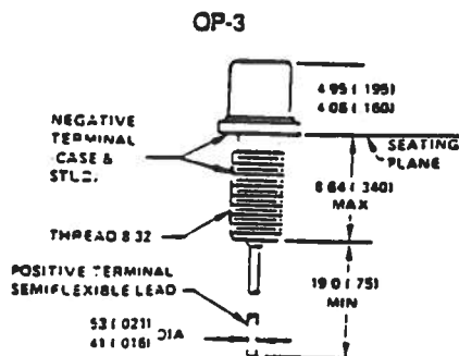
AVX-S3 INPUT ASSEMBLY (FOR OP-3 PACKAGE)
