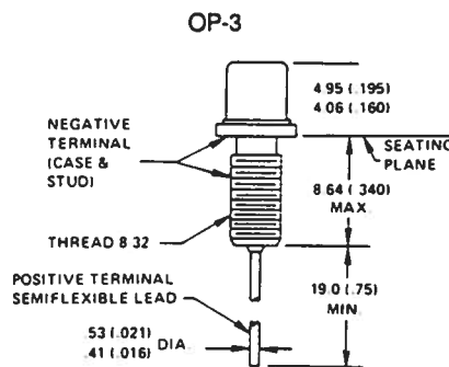
TYPICAL PACKAGES
