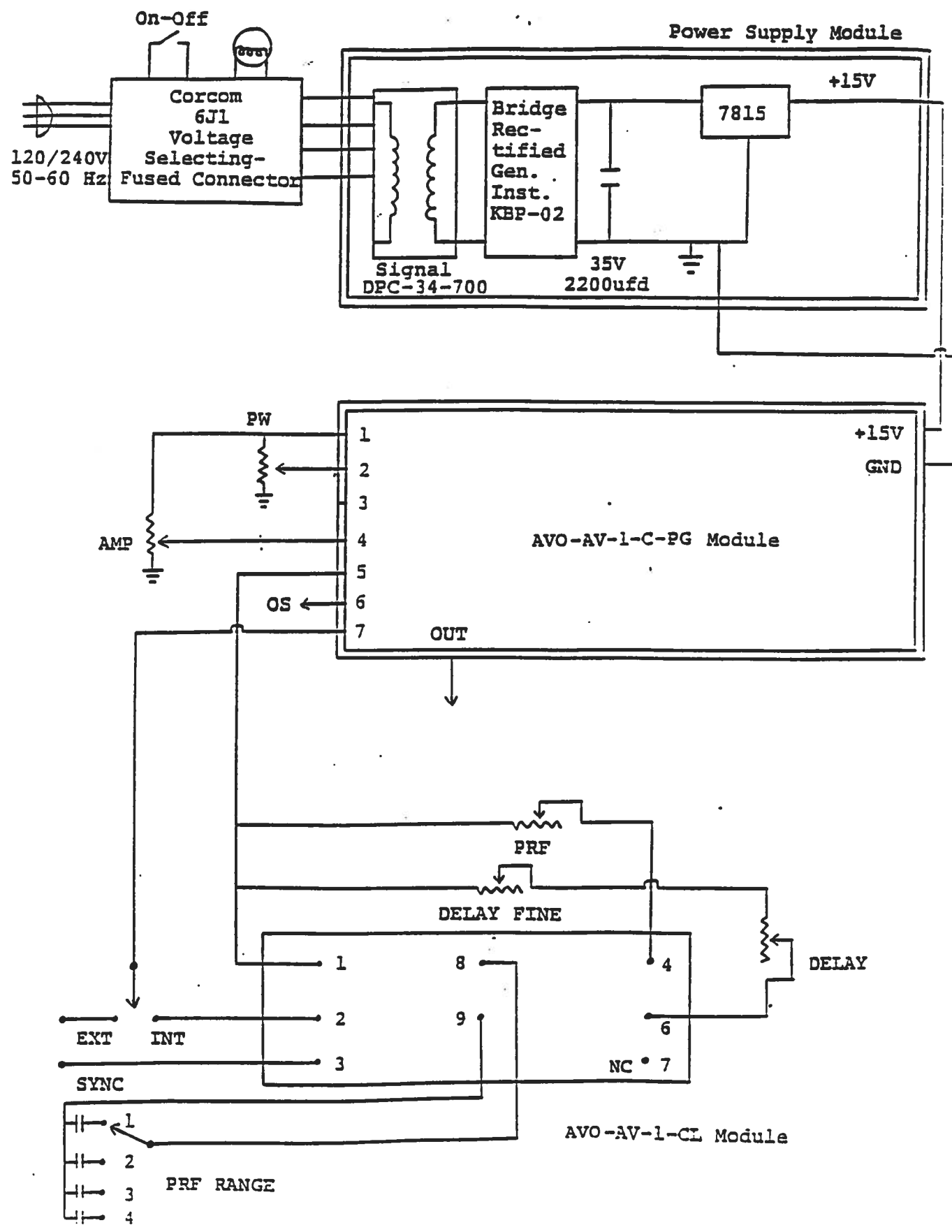
FIG. 5: SYSTEM BLOCK DIAGRAM
