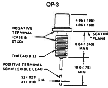
TYPICAL PACKAGES
