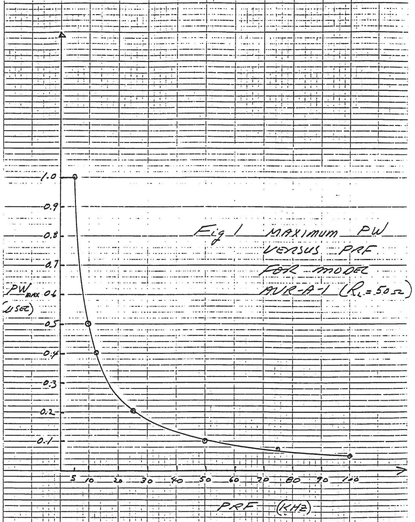
Fig. 1A: MAXIMUM PW VERSUS PRF FOR MODEL AVR-A-1 ( R_L = 50 \Omega )
