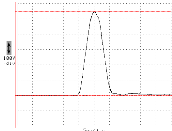
AVRK-3-B-P, 550V amplitude, 6 ns pulse width
