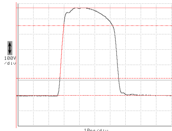
AVRK-3-B-P, 550V amplitude, 35 ns pulse width
