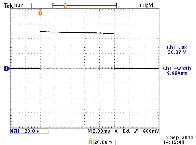
10 Hz, 10 ms, +50V, into 50 \Omega . 20V/div, 2 ms/div.
