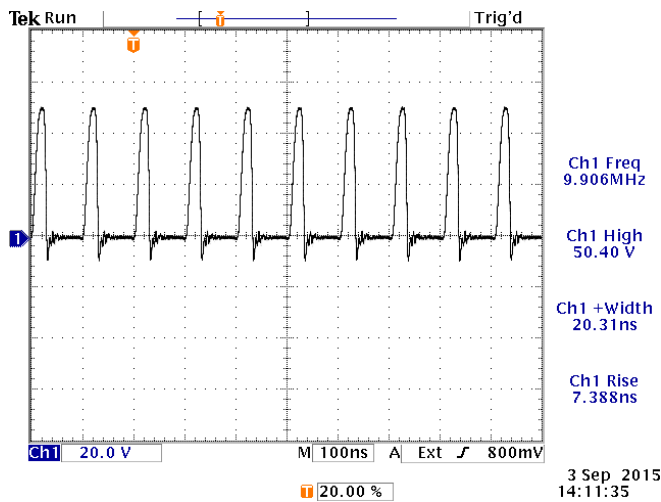
10 MHz, 20 ns, +50V, into 50 \Omega . 20V/div, 100 ns/div.
