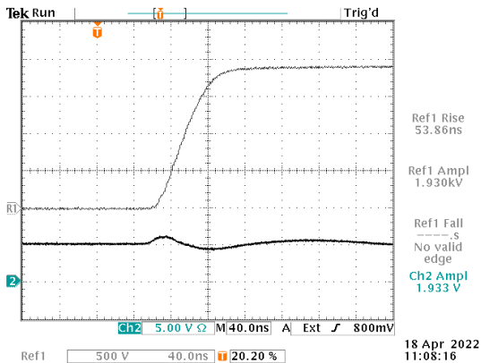
C = 1000 pF, t_{R10-90} = 53.86 ns
