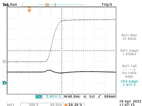
C = 820 pF, t_{R10-90} = 37.86 ns
