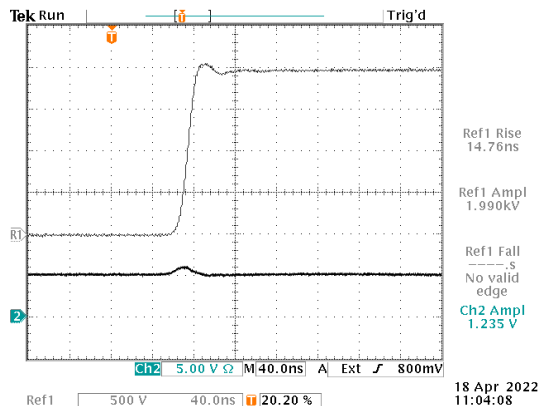
C = 150 pF, t_{R10-90} = 14.76 ns
