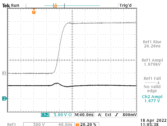
C = 450 pF, t_{R10-90} = 26.26 ns
