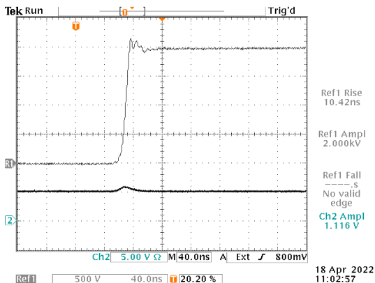
C = 0 pF, t_{R10-90} = 10.42 ns
