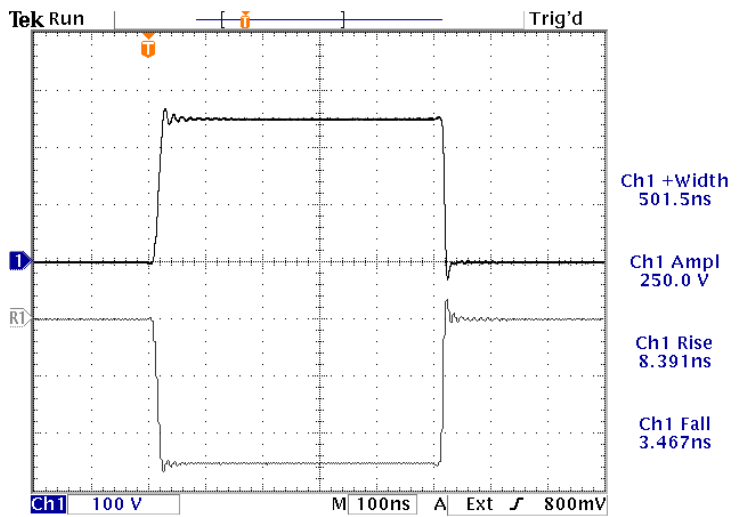
19 Jun 2018 09:44:51 Ref1 100 V 100ns 20.00 % 10 kHz, 500 ns, +250V and -250V into a 50Ω load. 100 V/div, 100 ns/div.
