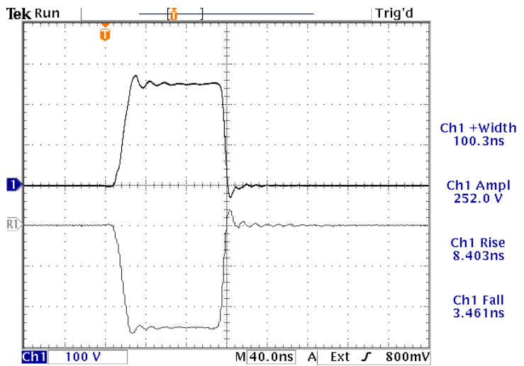
19 Jun 2018 09:43:47 Ref1 100 V 40.0ns 20.00 % 100 kHz, 100 ns, +250V and -250V into a 50Ω load. 100 V/div, 40 ns/div.
