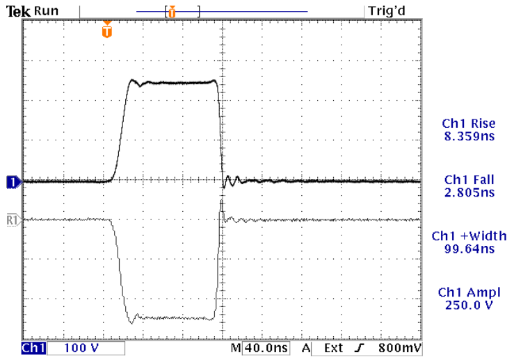
100 kHz, 100 ns, +250V and -250V into a 50Ω load. 100 V/div, 40 ns/div.
