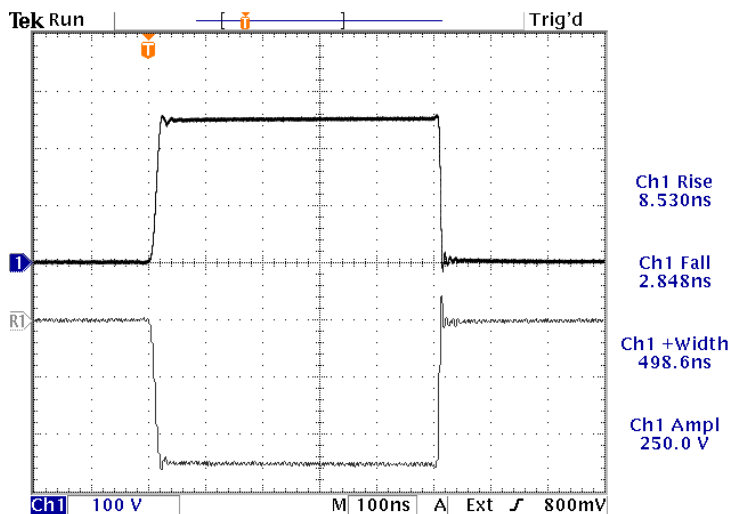
10 kHz, 500 ns, +250V and -250V into a 50Ω load. 100 V/div, 100 ns/div.
